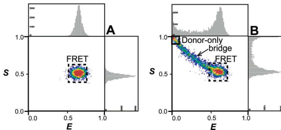
Figure 2. Simulated single-molecule 2D E-S ALEX histograms of (A) pure doubly labeled FRET species (dashed black square) and (B) a scenario where the acceptor is partially bleached, showing donor only (solid black square), FRET species (dashed black square), and “bridge” events.
